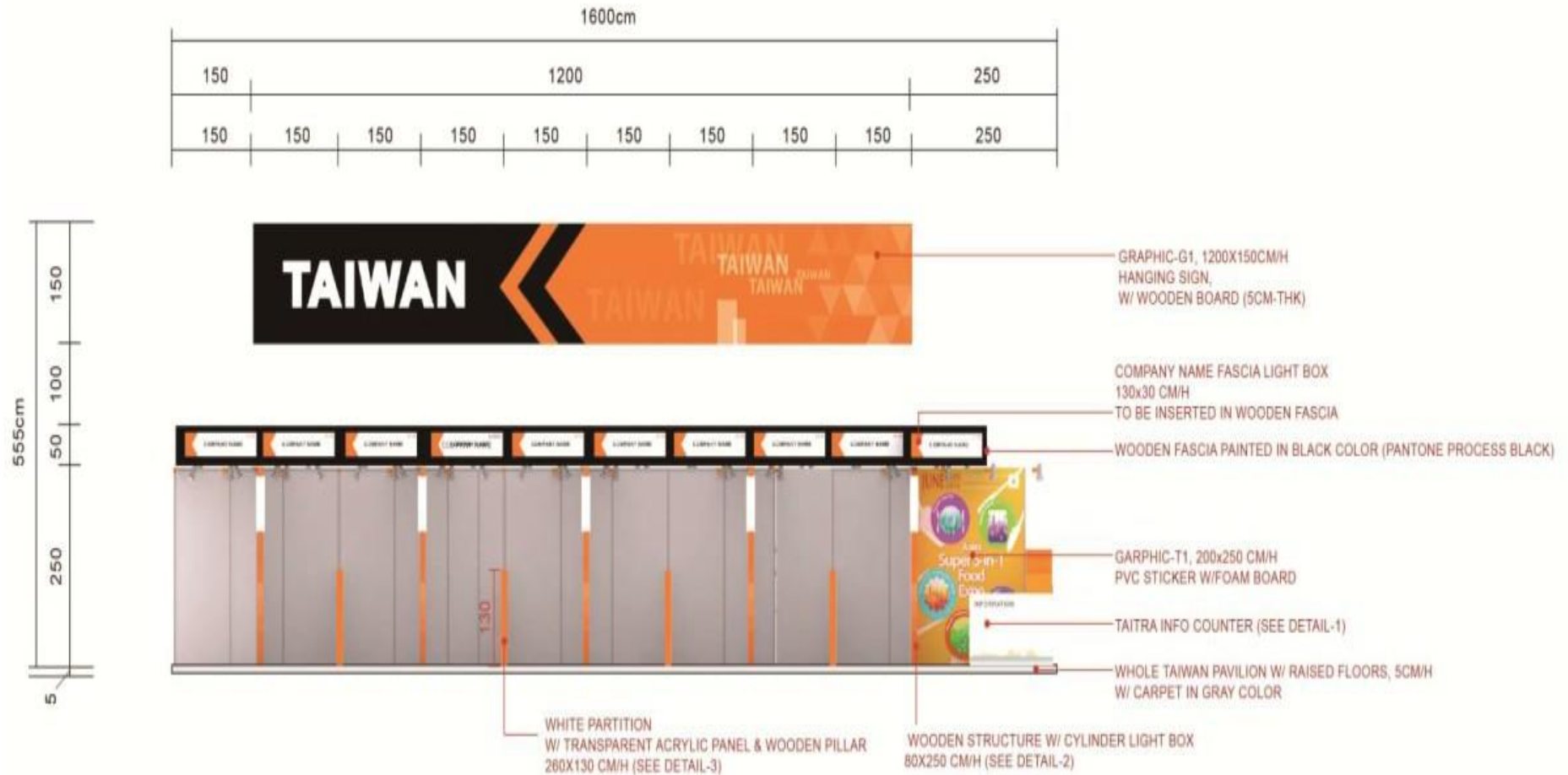
① ELEVATION PLAN S:1 / 100
